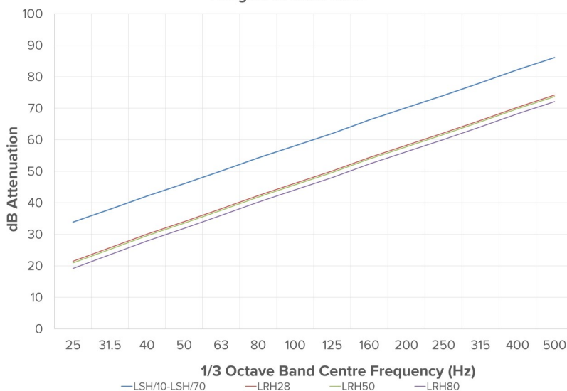
Structural Force Attenuation of LSH and LRH Acoustic Ceiling Hangers at rated load.
