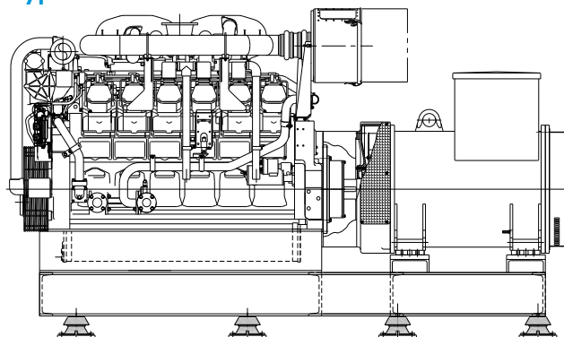
TSC T20 isolators used on a generating set
